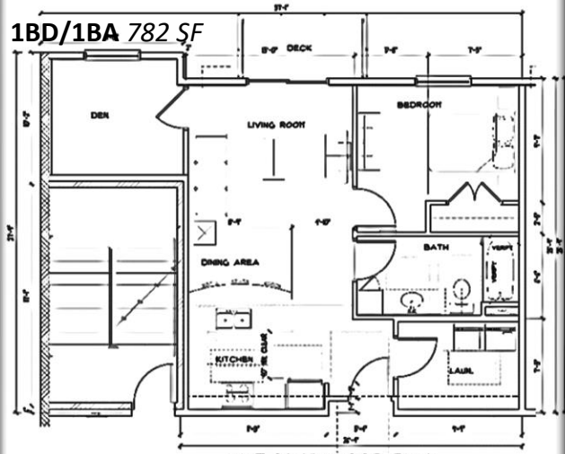
UNIT "A3" FLOOR PLAN SCALE 1/4" = 1'-0" TYPE "B" 782 SF 1 BED 1 BATH (12) TOTAL
