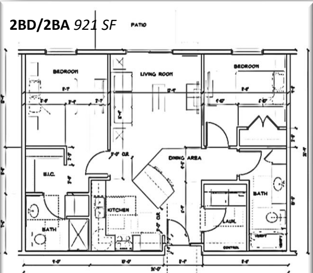
UNIT "B" FLOOR PLAN SCALE 1/4" = 1'-0" TYPE "B" 921 SF 2 BED 2 BATH (10) TOTAL (10) W/ DECKS
