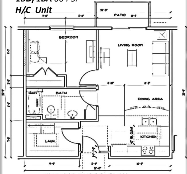
UNIT "A" FLOOR PLAN SCALE 1/4" = 1'-0" TYPE "B" 664 SF 1 BED 1 BATH (10) TOTAL (10) W/ DECKS
